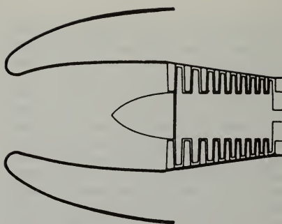
FIGURE 2-21. Divergent subsonic inlet duct.
